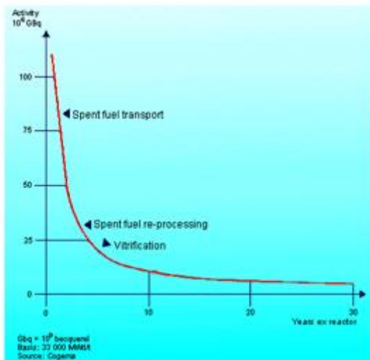
Decay in radioactivity of fission products – one tonne of spent PWR fuel
