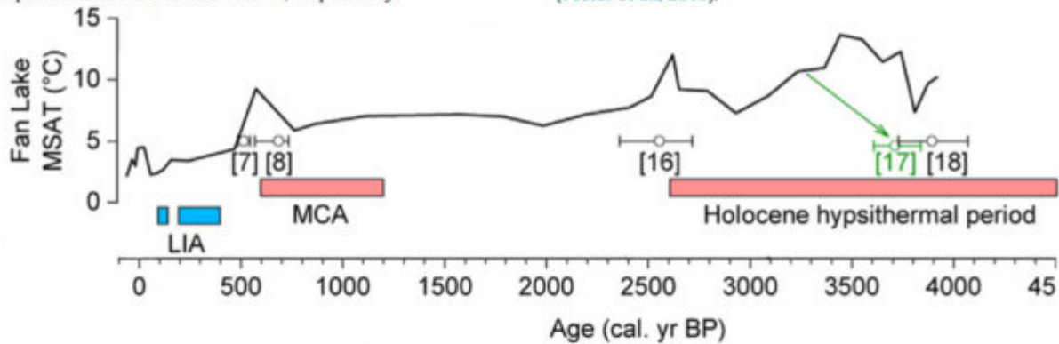
Mean summer air temperature (MSAT) record reconstructed from Fan Lake (Foster et al., 2016). Here the chronological anchor points for these temperature peaks used by Strother et al. (2015) are also shown along with their ID numbers (7, 8, 16, and 18). The green radiocarbon dating point (ID number 17) was rejected in the original age-depth model, but if used, the horizon of 3250 cal yr BP would be anchored to an older age, pulling this section of the MSAT curve rightward in the Bayesian age-depth modeling. The red horizontal bars below show the periods of past warm intervals by Foster et al. (2016) based on their multi-proxy dataset. MCA—Medieval Climate Anomaly.
