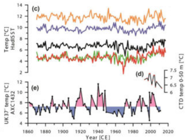
(c) Average July–October HadISST temperature (Rayner et al., 2003), with the color code for each plot being related to the color of each box shown on the map in (a). (d) average CTD temperature within the uppermost 50 m from (b). (e) BAYSPLINE AIsST record from Nørre Skjoldungesund starting in 1860. Colors indicate variation from the average value 7.23°C.
