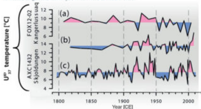
Figure 6: (a)–(c) AIsST reconstructions from three fjords in SE-Greenland. (a) Kangerlussuaq Fjord, core FOX12-02 (Vermassen et al., 2019), (b) Sermilik Fjord, core ER07 (Andresen et al., 2017) and (c) Nørre Skjoldungesund, core AXC1432 (this study, using the BAYSPLINE calibration). Colors indicate the variance from the individual average.
