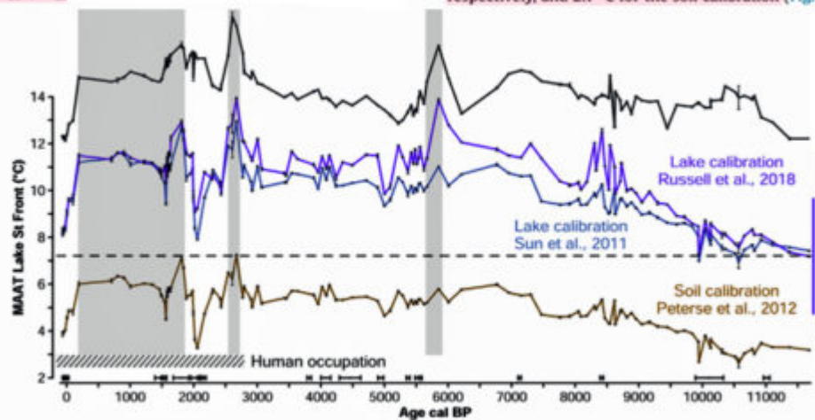
Mean annual air temperatures (MAAT) reconstructed with Sun et al. (2011, blue curve), Russell et al. (2018, purple curve) and Peterse et al. (2012, brown curve) calibrations compared with the present mean annual temperature at St Front (black dashed line)
