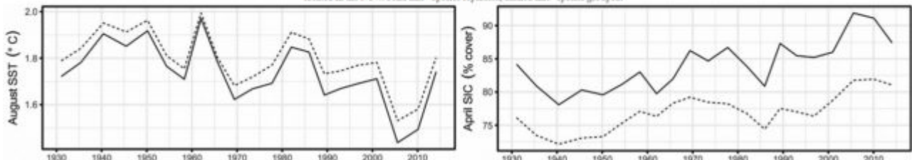
Fig. 6 Quantitative reconstructions of past aSST and aSIC from core AMD15-CASQ1-BC located in the NORG. Solid line = species separated, dashed line = species grouped.
