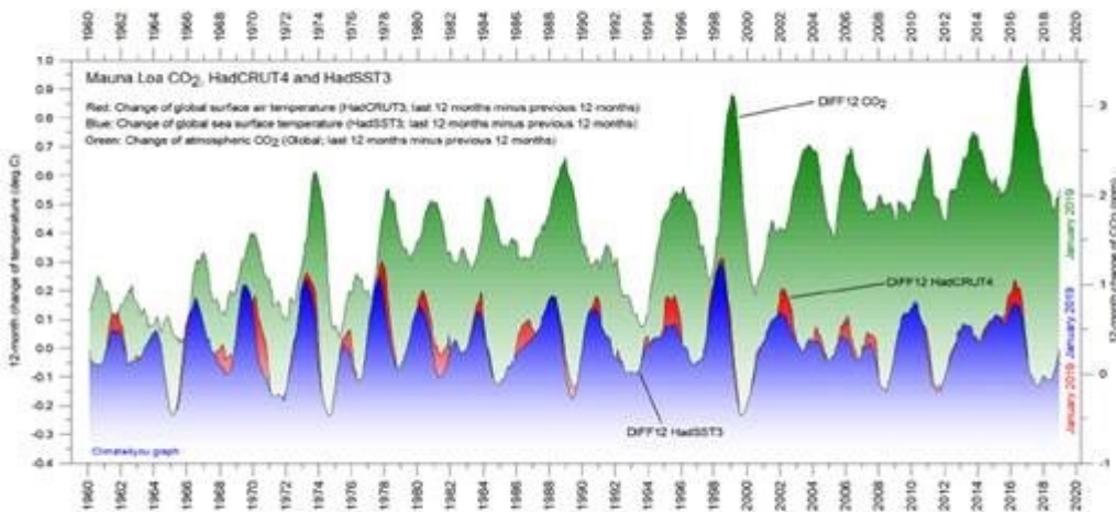
12-month change of global atmospheric CO 2 concentration (Mauna Loa; green), global sea surface temperature (HadSST3; blue) and global surface air temperature (HadCRUT4; red dotted). All graphs are showing monthly values of DIFF12, the difference between the average of the last 12 months and the average for the previous 12 months for each data series.
